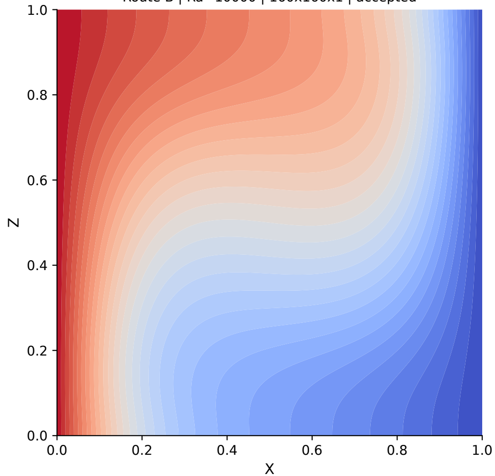
B-Ra1e4-fine Route B | Ra=10000 | 160x160x1 | accepted
