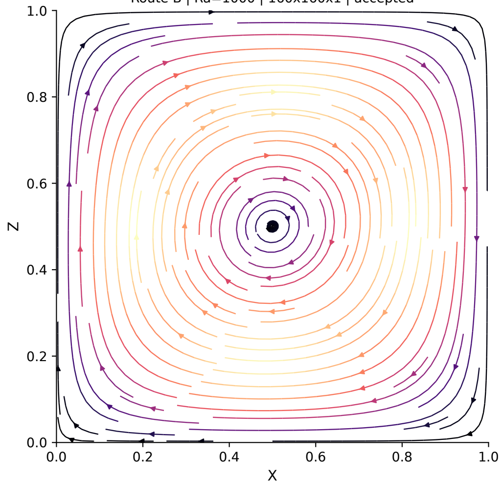
B-Ra1e3-fine Route B | Ra=1000 | 160 \times 160 \times 1 | accepted
