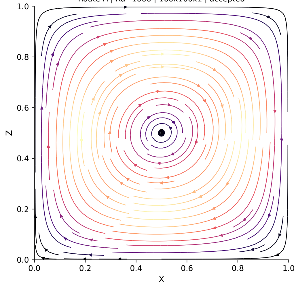
A-Ra1e3-fine Route A | Ra=1000 | 160 \times 160 \times 1 | accepted
