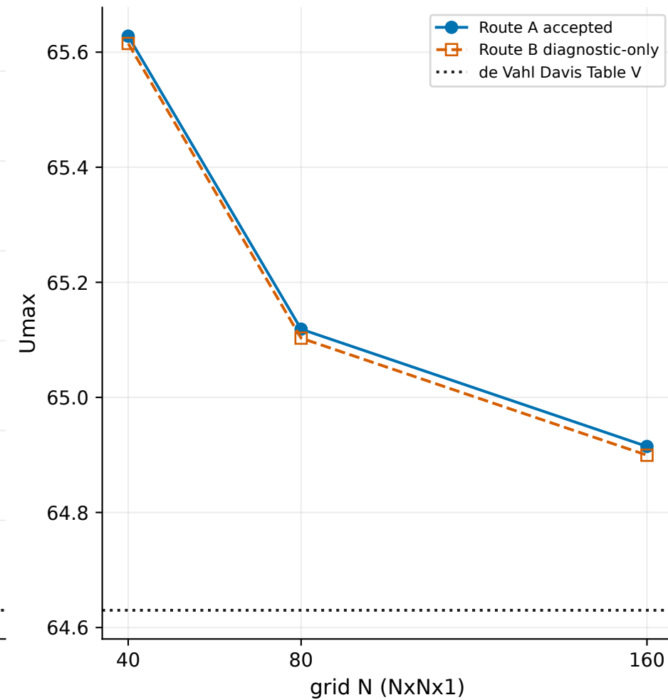
Grid dependence | Ra=1e+06 (Gate F status retained)
