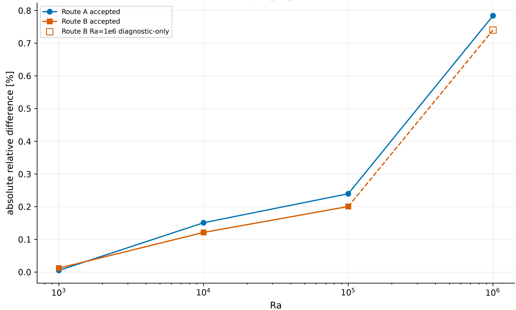
Fine 160x160x1 | Nu_bar_cavity | vs Table V
