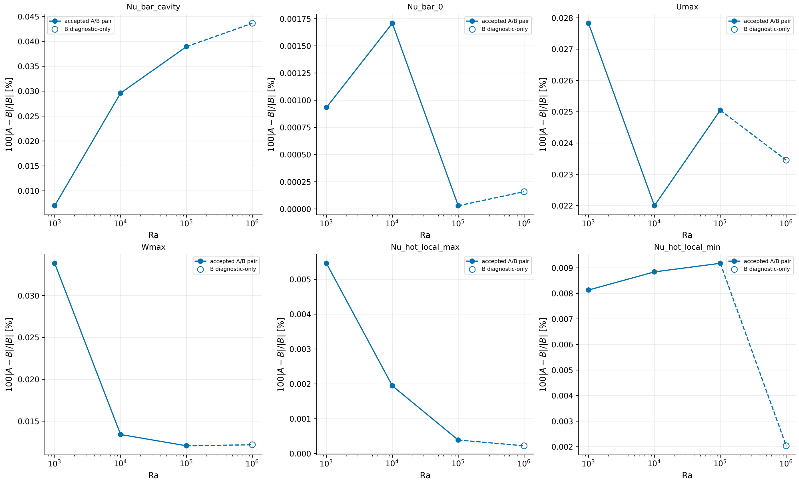
Fine 160x160x1: model/formulation comparison (not an error bound)
