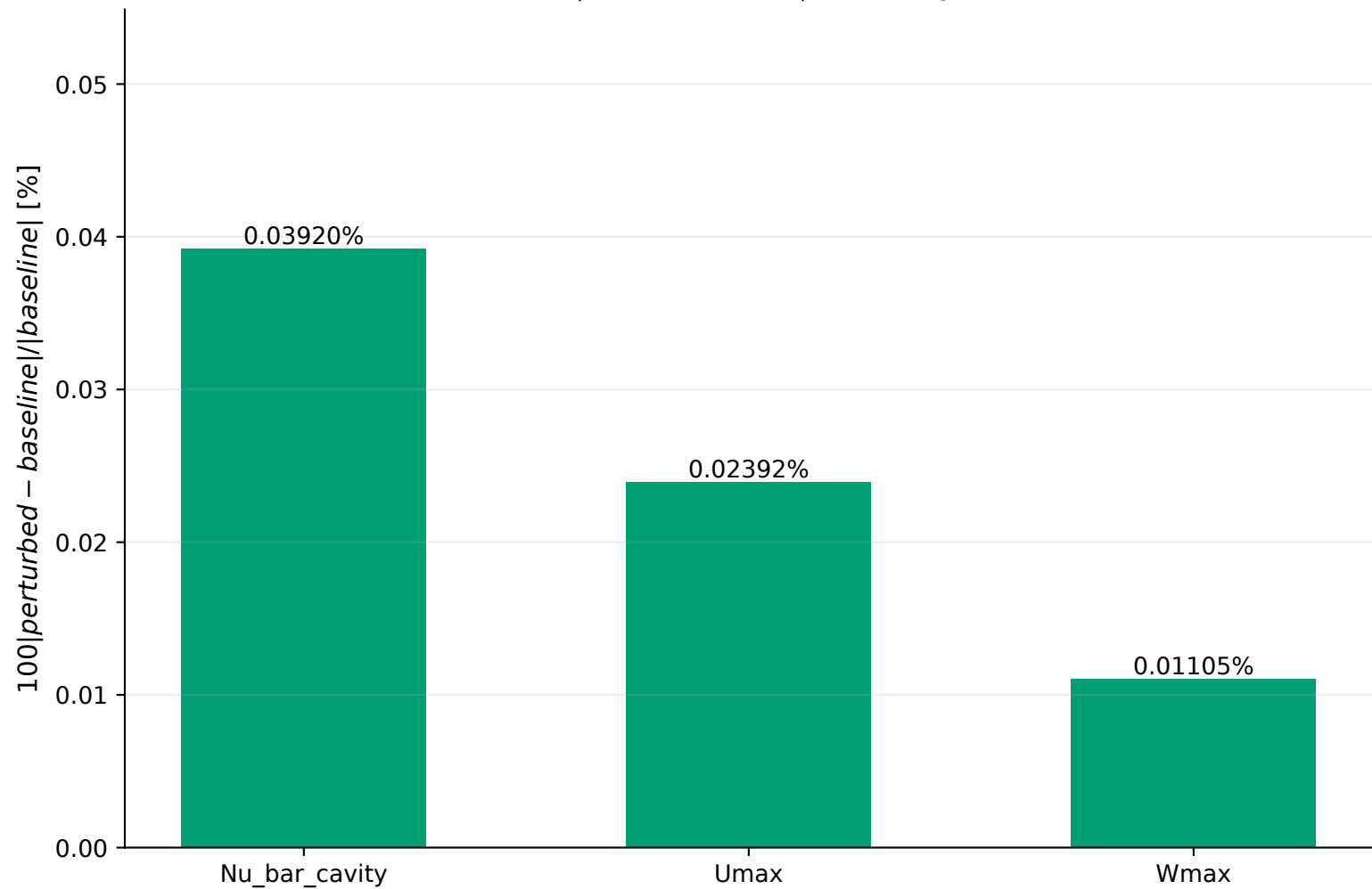
Gate H | fixed 160x160x1 | beta / 10, g x 10
