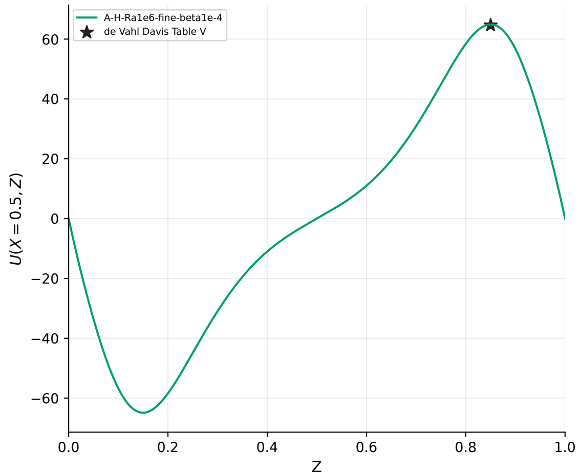
A-H-Ra1e6-fine-beta1e-4 Route A | Ra=1e+06 | 160x160x1 | accepted
