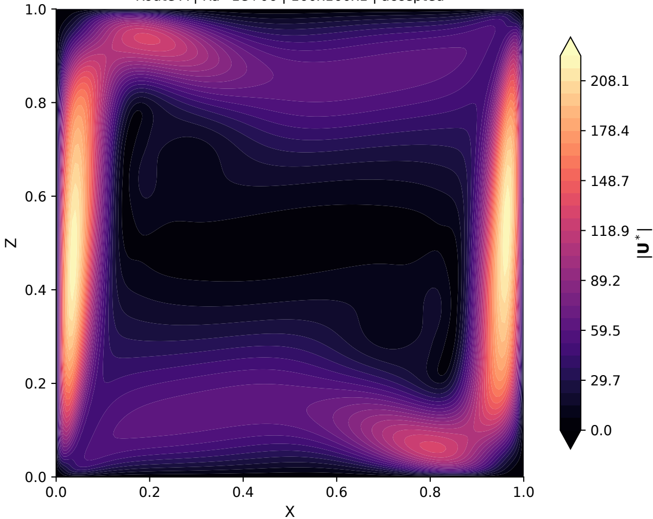
A-H-Ra1e6-fine-beta1e-4 Route A | Ra=1e+06 | 160 \times 160 \times 1 | accepted
