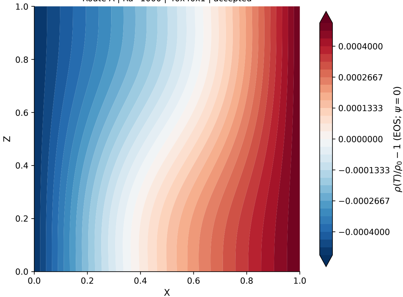
A-Ra1e3-coarse Route A | Ra=1000 | 40x40x1 | accepted
