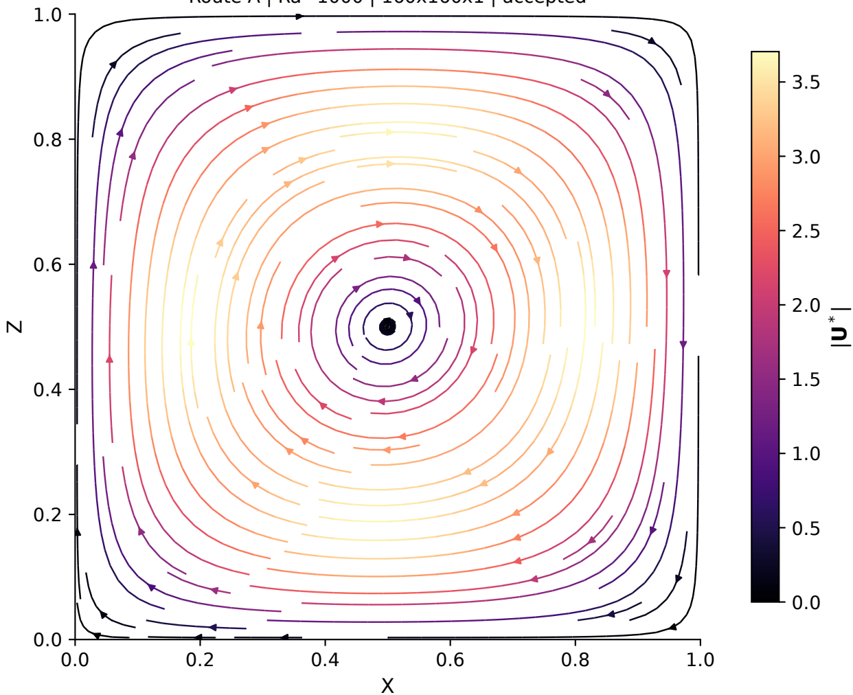
A-Ra1e3-fine Route A | Ra=1000 | 160x160x1 | accepted
