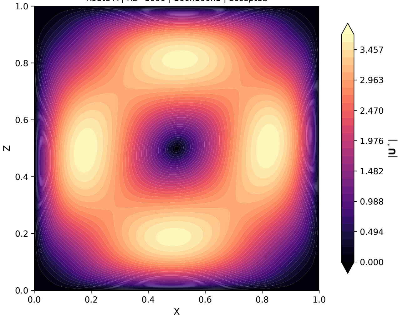
A-Rale3-fine Route A | Ra=1000 | 160x160x1 | accepted
