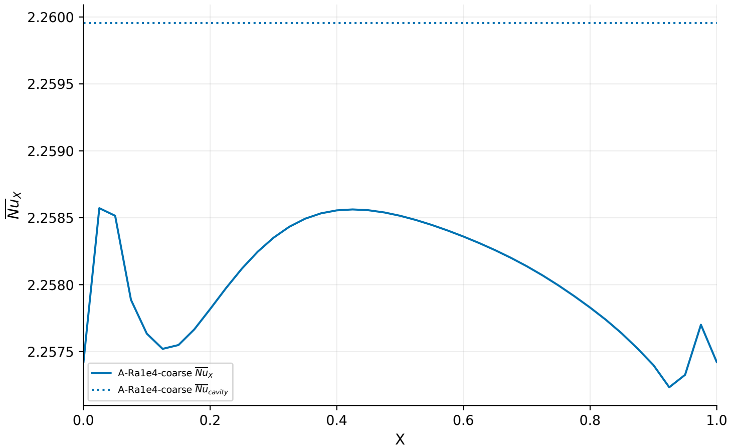
A-Ra1e4-coarse Route A | Ra=10000 | 40x40x1 | accepted A: interpolated cell U
