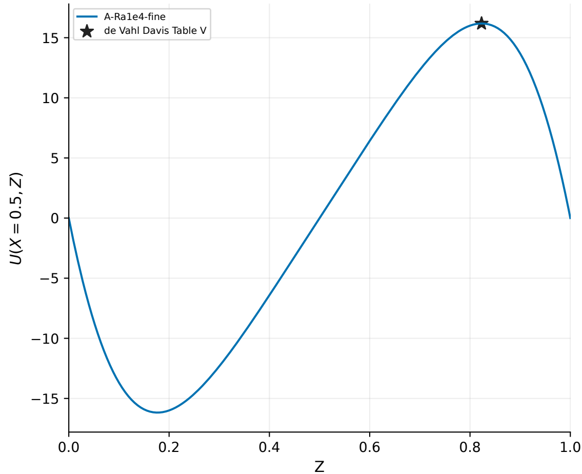
A-Ra1e4-fine Route A | Ra=10000 | 160x160x1 | accepted
