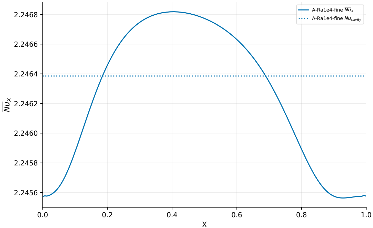
A-Ra1e4-fine Route A | Ra=10000 | 160x160x1 | accepted A: interpolated cell U
