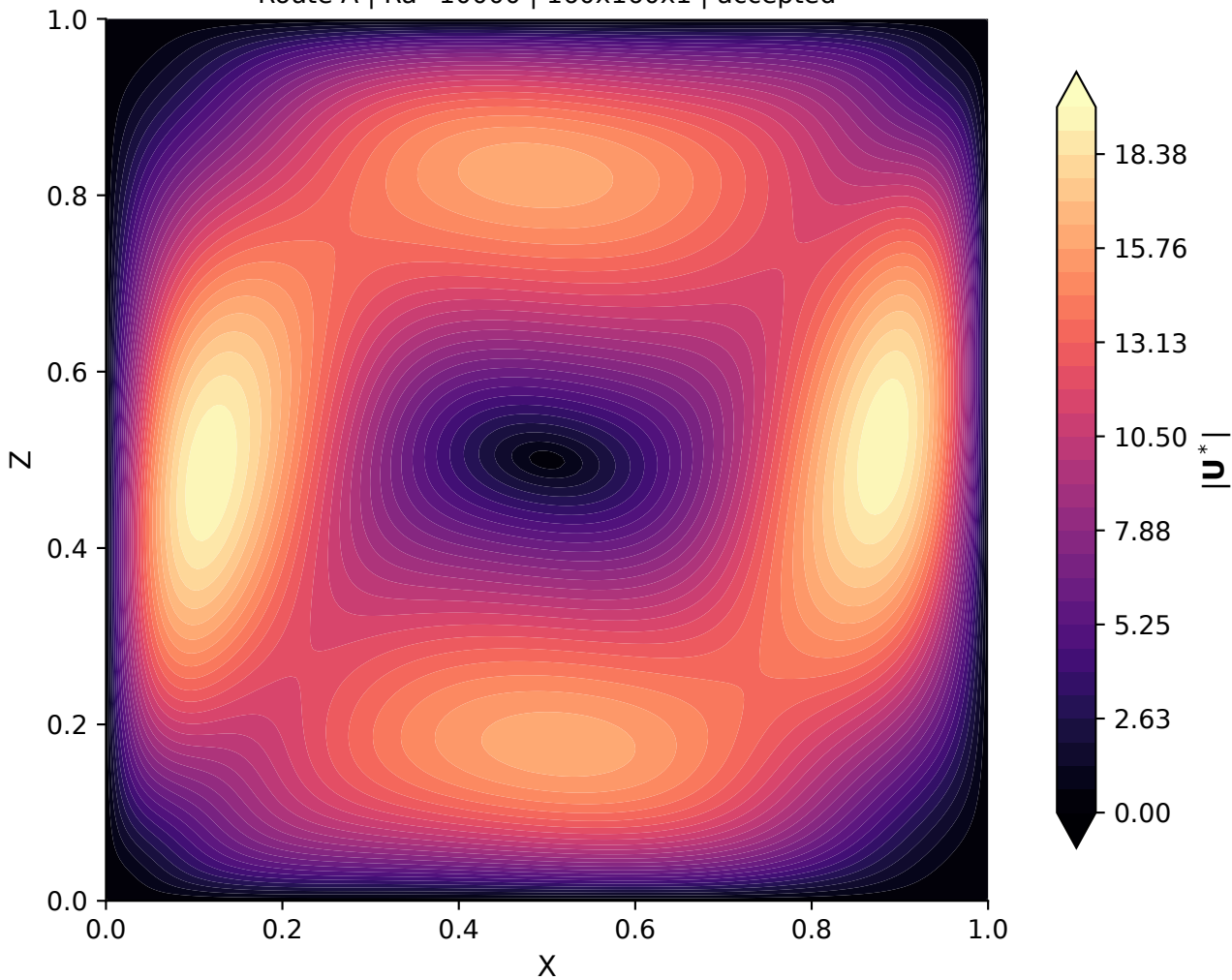
A-Ra1e4-fine Route A | Ra=10000 | 160x160x1 | accepted
