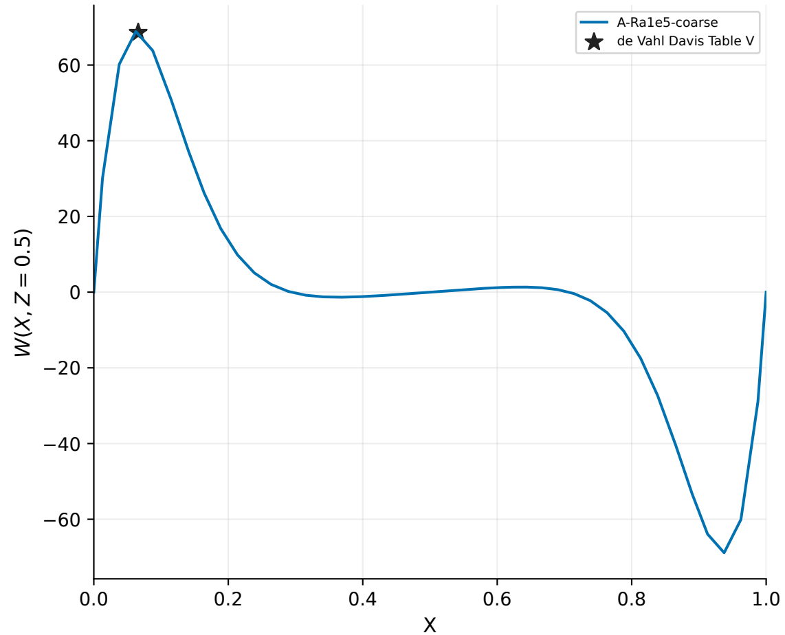
A-Ra1e5-coarse Route A | Ra=100000 | 40x40x1 | accepted
