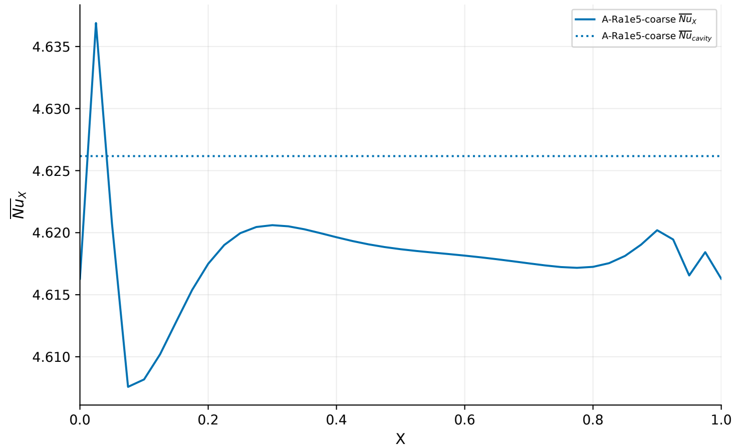
A-Ra1e5-coarse Route A | Ra=100000 | 40x40x1 | accepted A: interpolated cell U
