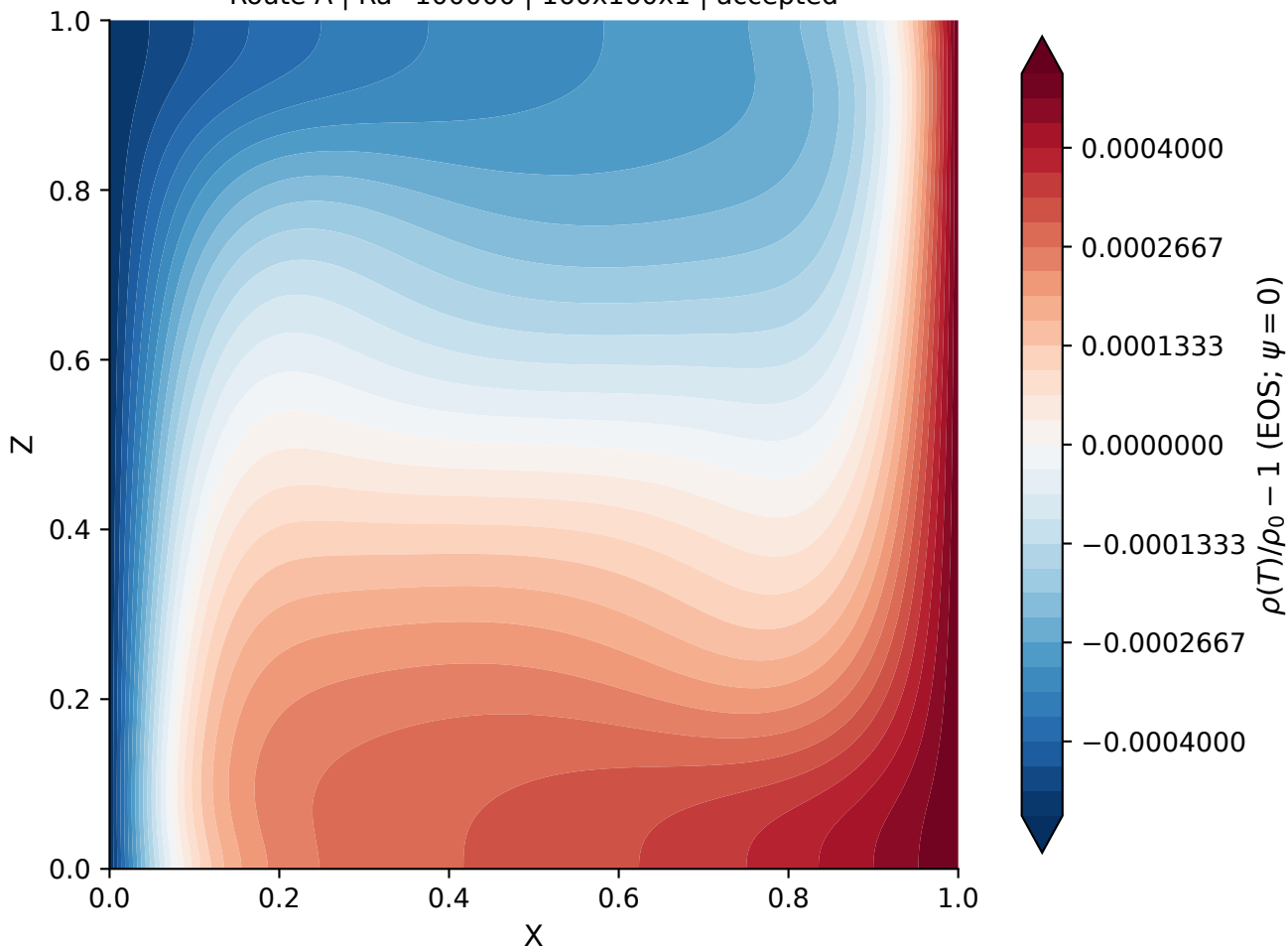
A-Ra1e5-fine Route A | Ra=100000 | 160x160x1 | accepted
