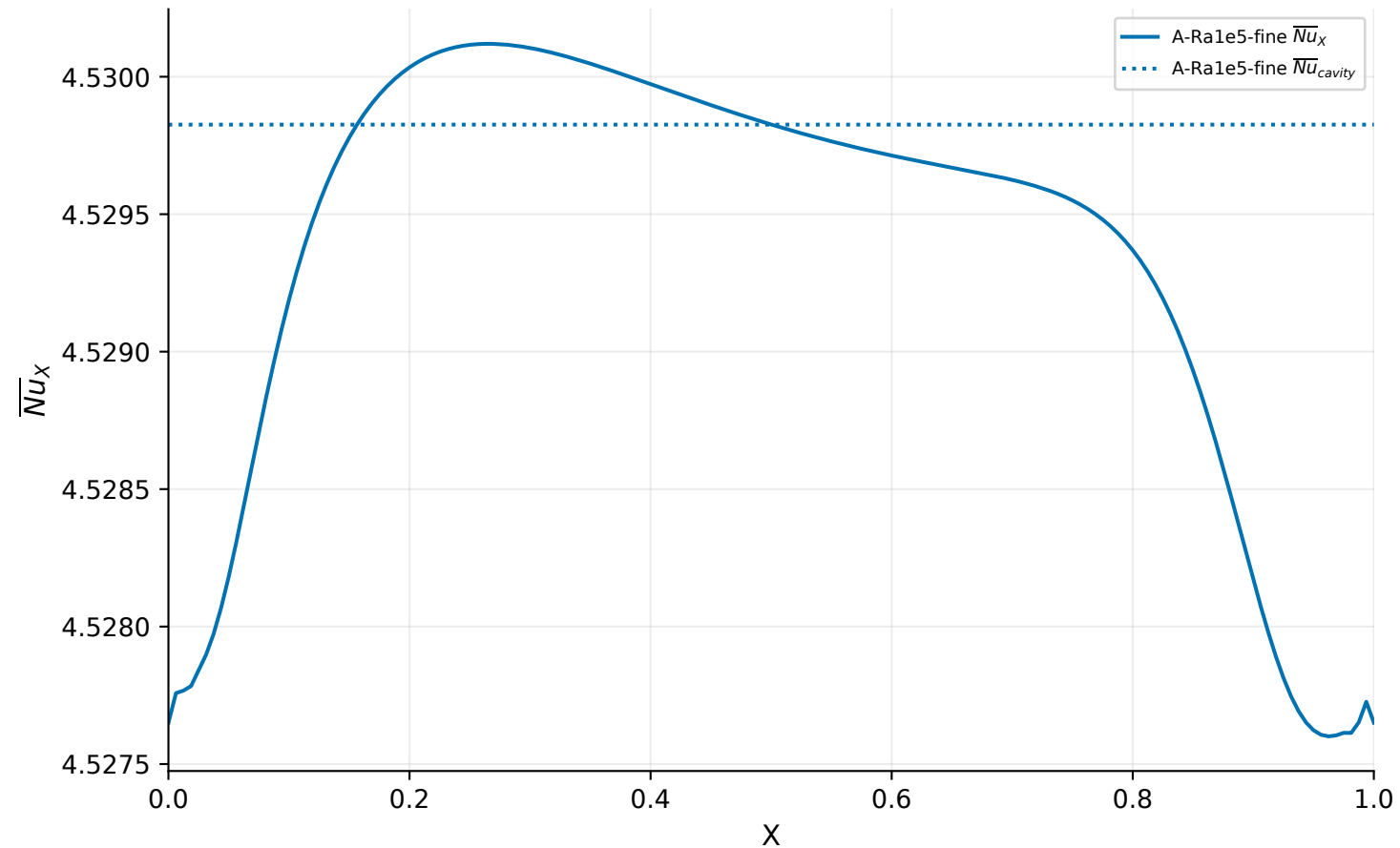
A-Ra1e5-fine Route A | Ra=100000 | 160x160x1 | accepted A: interpolated cell U
