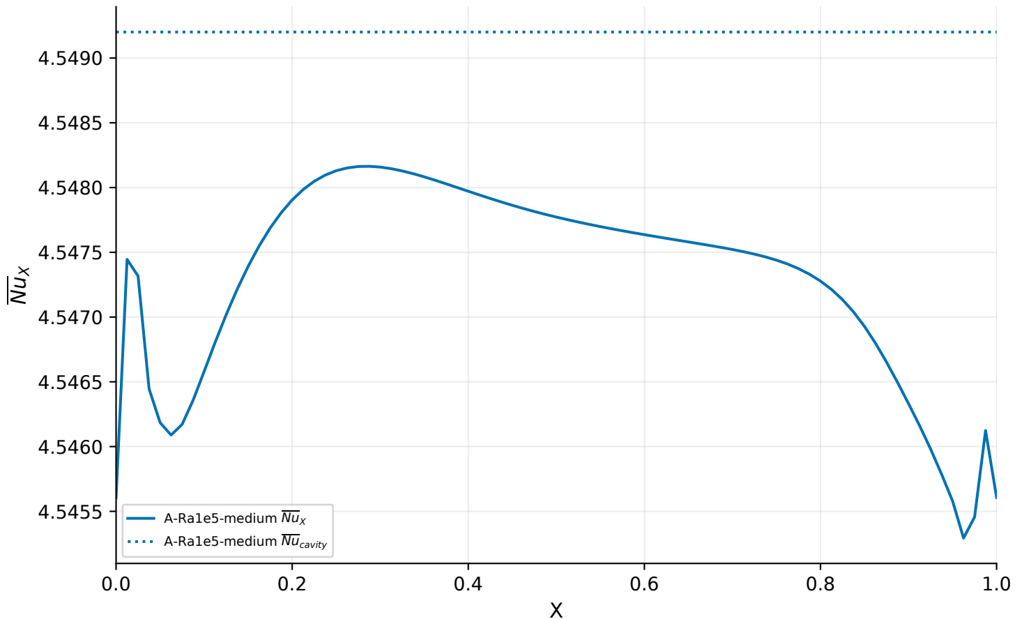
A-Ra1e5-medium Route A | Ra=100000 | 80x80x1 | accepted A: interpolated cell U
