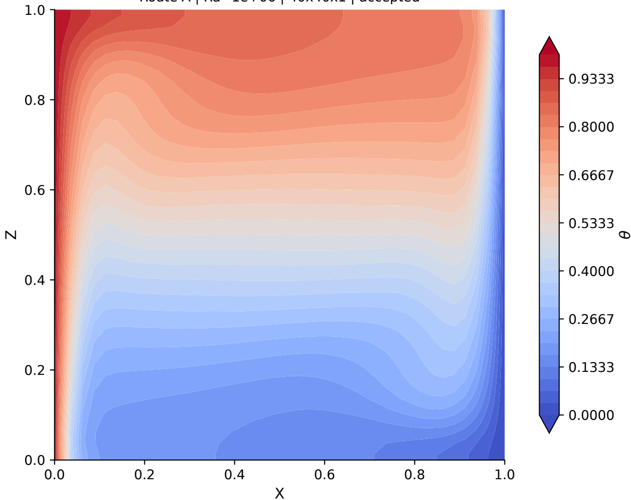
A-Ra1e6-coarse Route A | Ra=1e+06 | 40x40x1 | accepted
