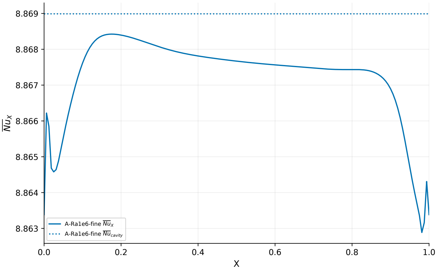
A-Ra1e6-fine Route A | Ra=1e+06 | 160x160x1 | accepted A: interpolated cell U
