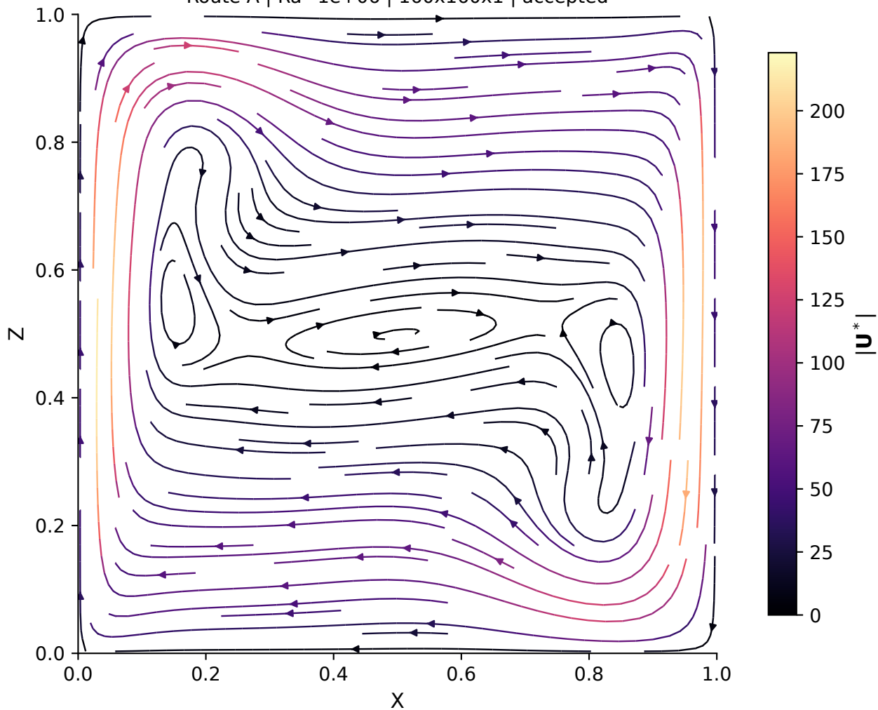
A-Ra1e6-fine Route A | Ra=1e+06 | 160 \times 160 \times 1 | accepted
