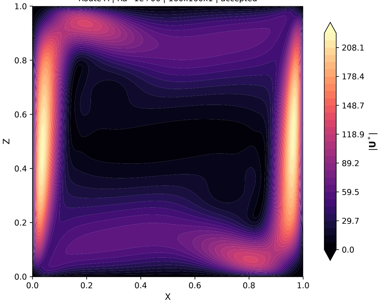
A-Ra1e6-fine Route A | Ra=1e+06 | 160x160x1 | accepted
