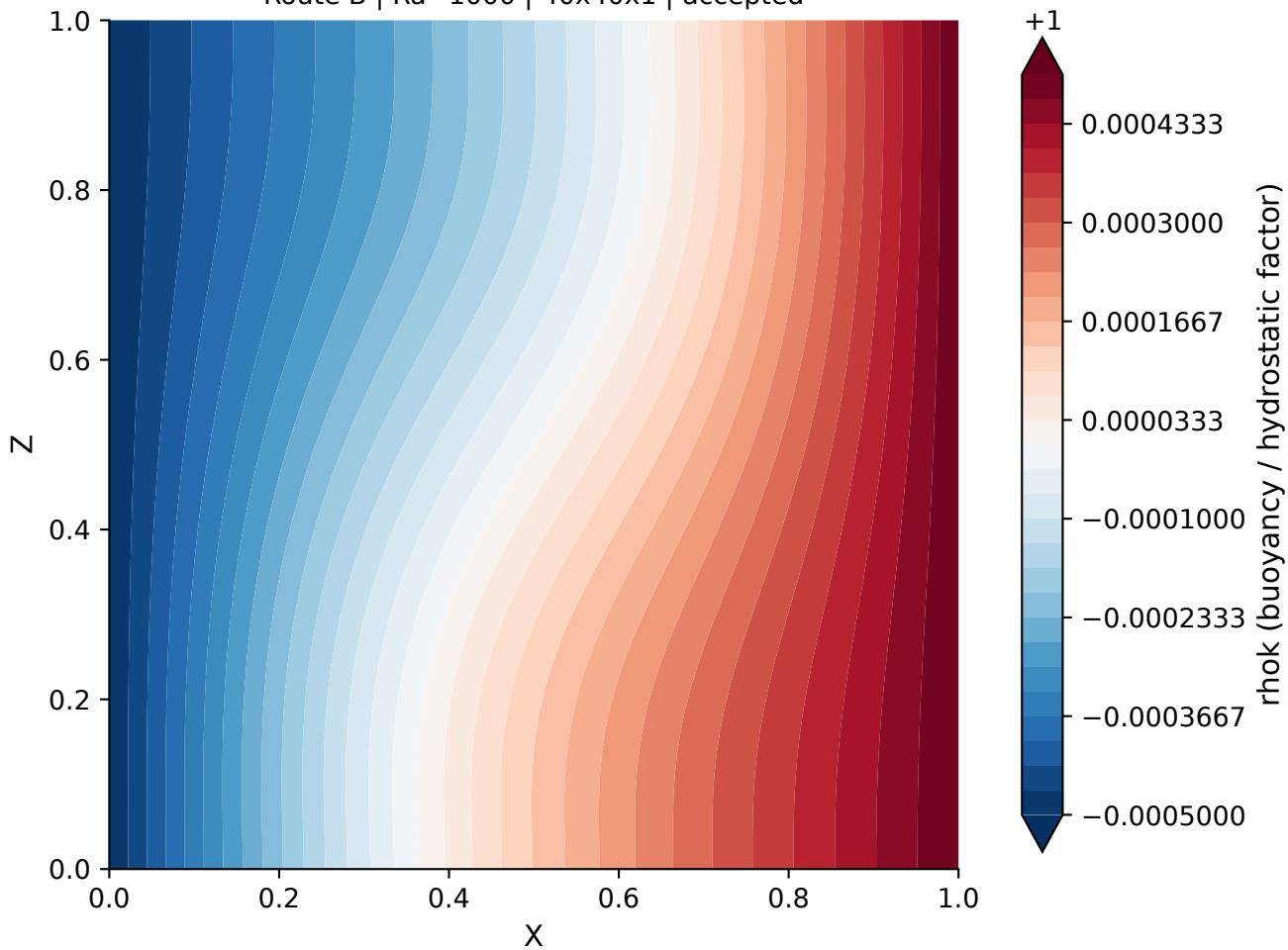
B-Ra1e3-coarse Route B | Ra=1000 | 40x40x1 | accepted
