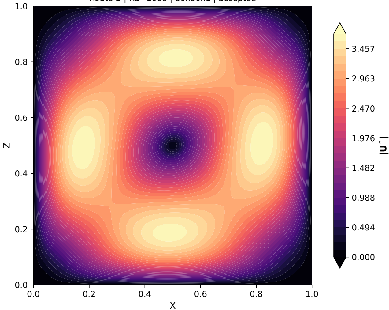
B-Ra1e3-medium Route B | Ra=1000 | 80x80x1 | accepted
