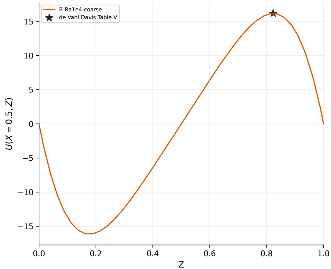
B-Ra1e4-coarse Route B | Ra=10000 | 40x40x1 | accepted
