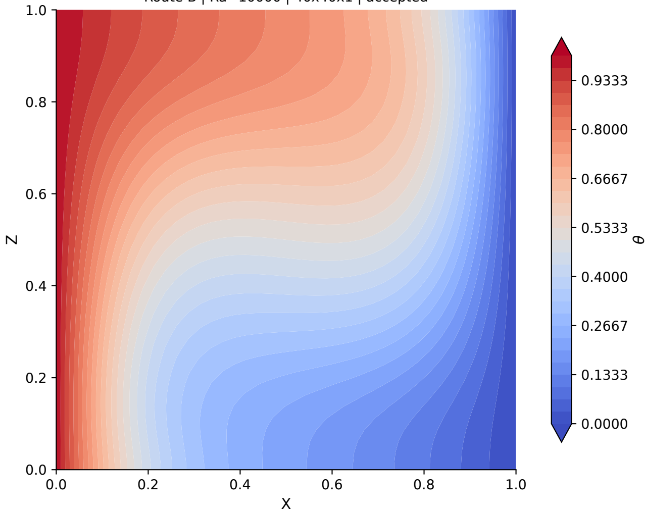
B-Ra1e4-coarse Route B | Ra=10000 | 40x40x1 | accepted
