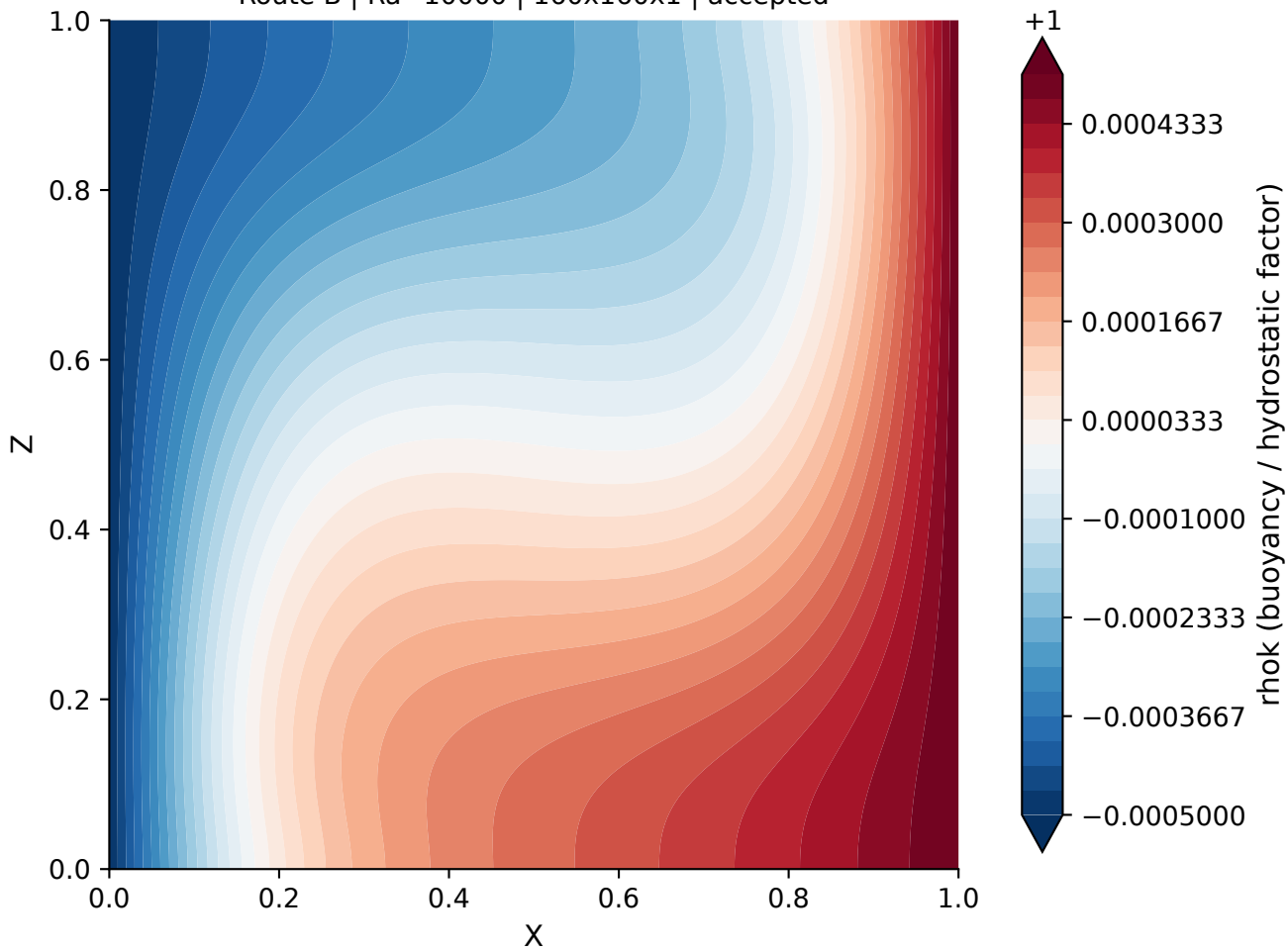
B-Rale4-fine Route B | Ra=10000 | 160x160x1 | accepted
