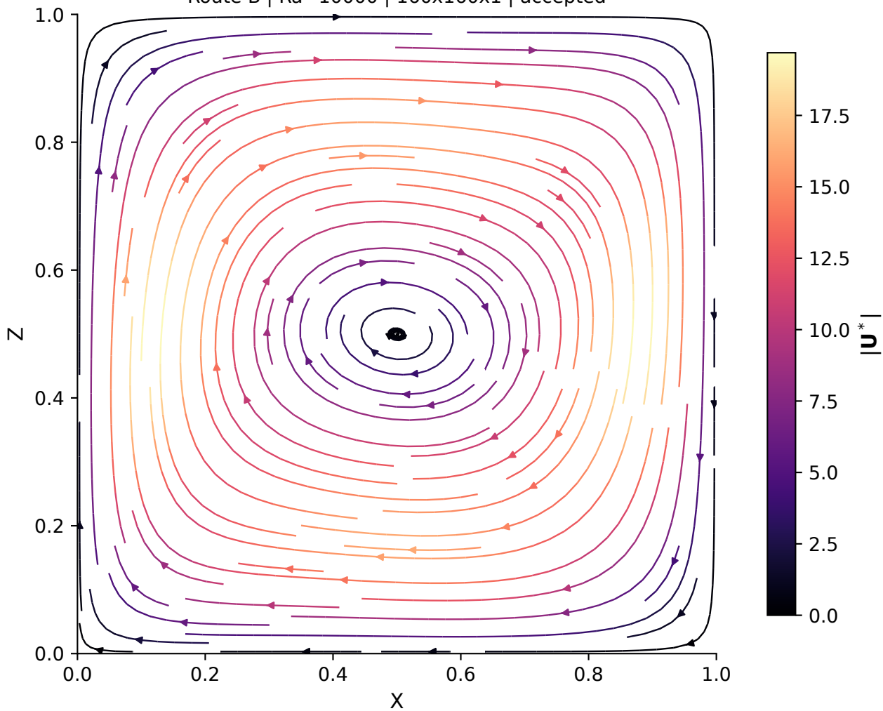
B-Ra1e4-fine Route B | Ra=10000 | 160x160x1 | accepted
