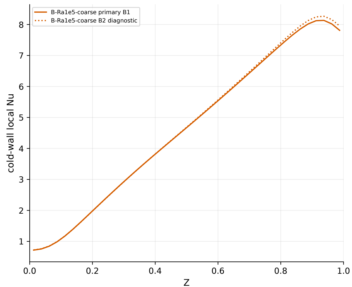
B-Ra1e5-coarse Route B | Ra=100000 | 40x40x1 | accepted
