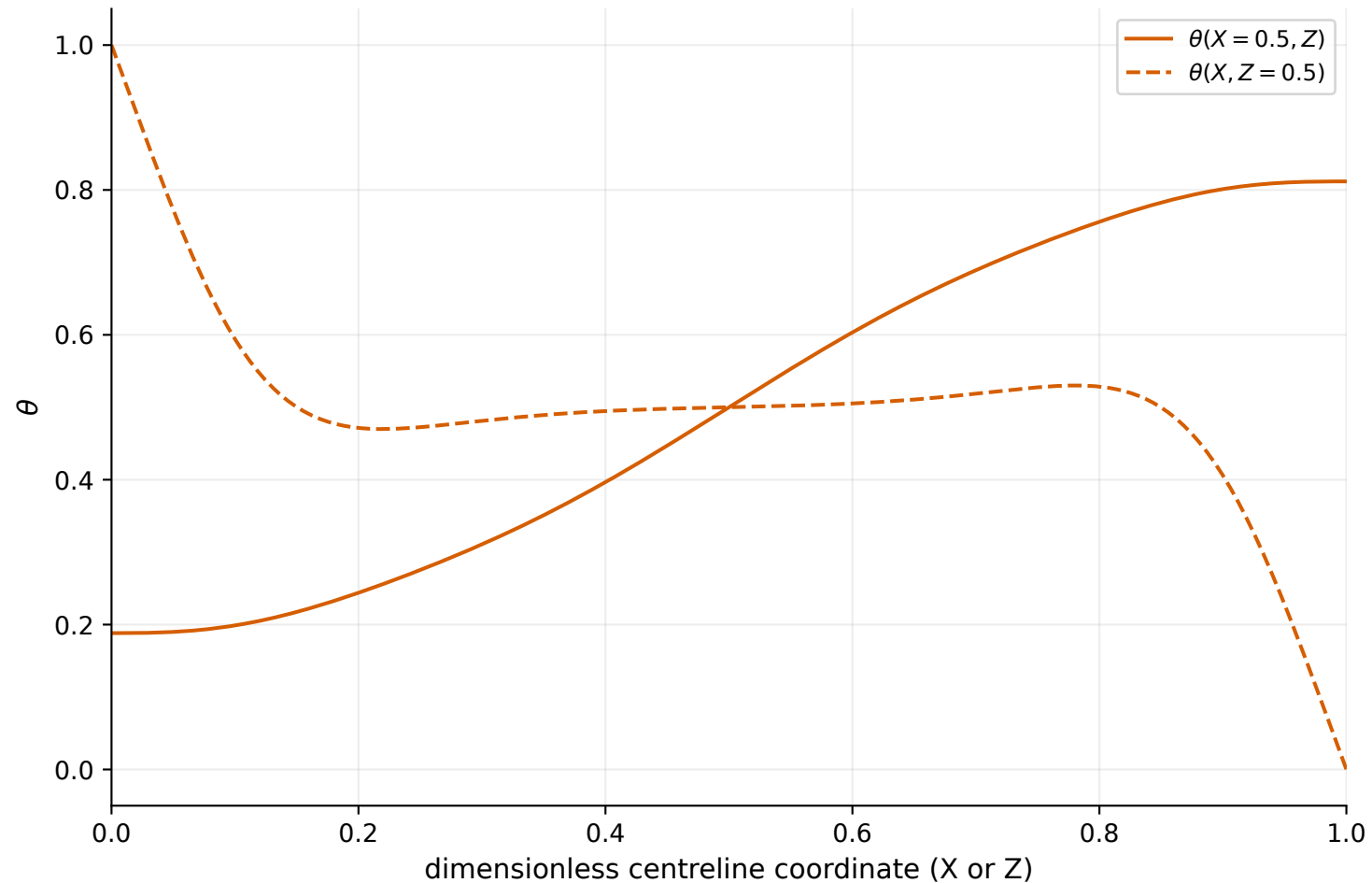
B-Ra1e5-fine Route B | Ra=100000 | 160x160x1 | accepted
