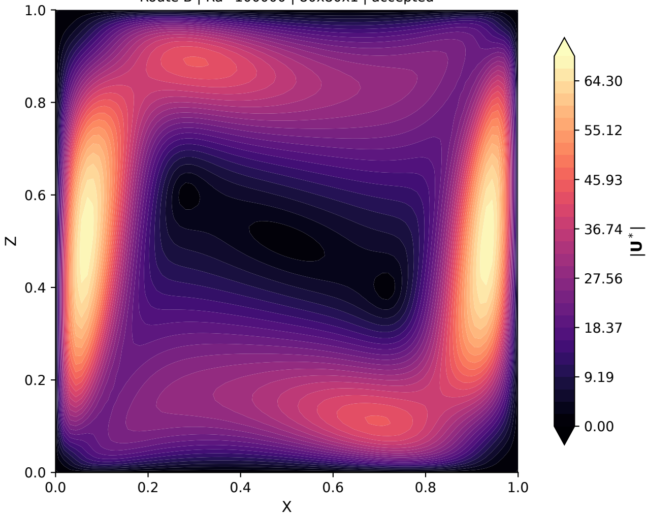
B-Ra1e5-medium Route B | Ra=100000 | 80x80x1 | accepted
