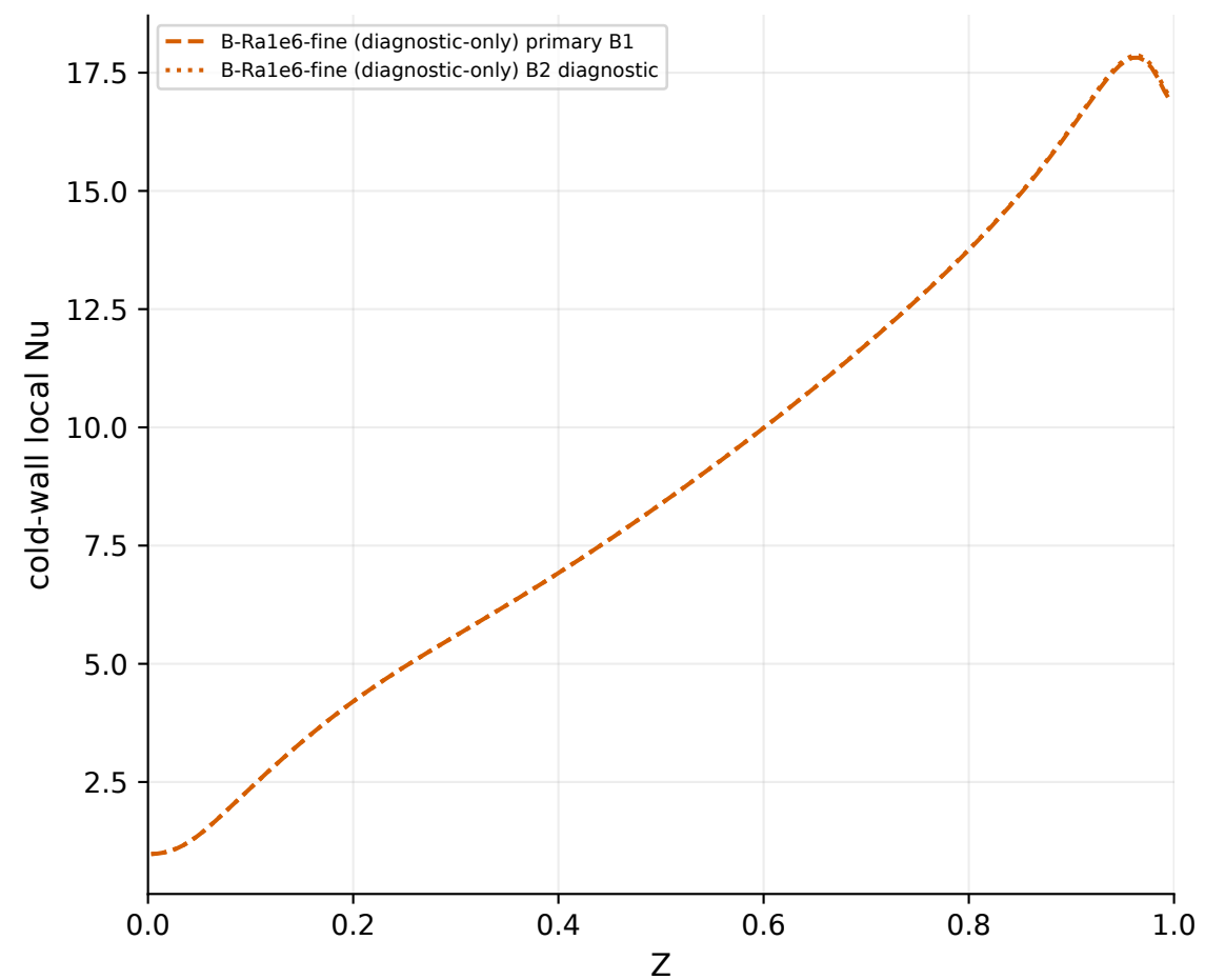
B-Ra1e6-fine Route B | Ra=1e+06 | 160x160x1 | diagnostic-only / unaccepted
