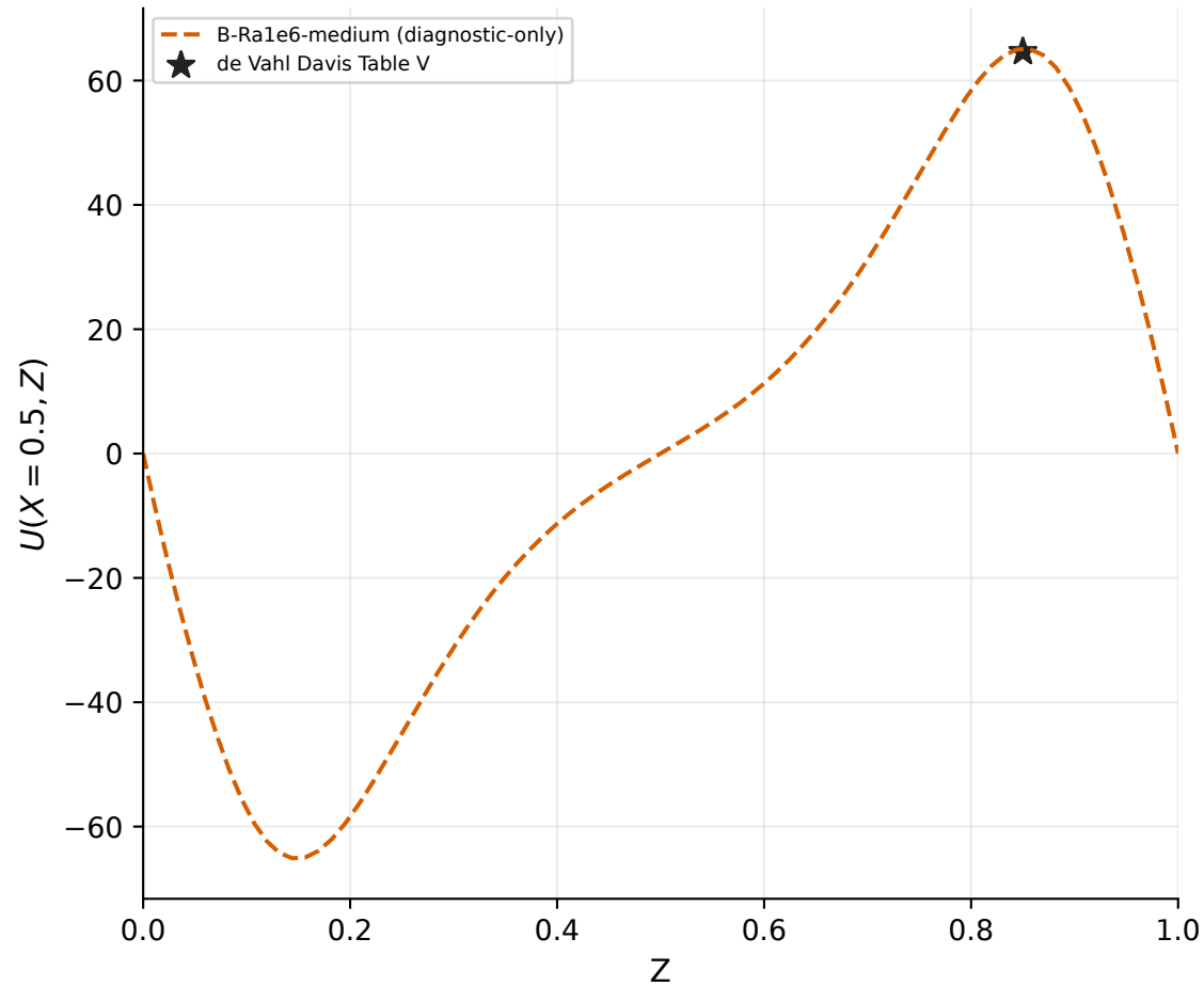
B-Ra1e6-medium Route B | Ra=1e+06 | 80x80x1 | diagnostic-only / unaccepted
