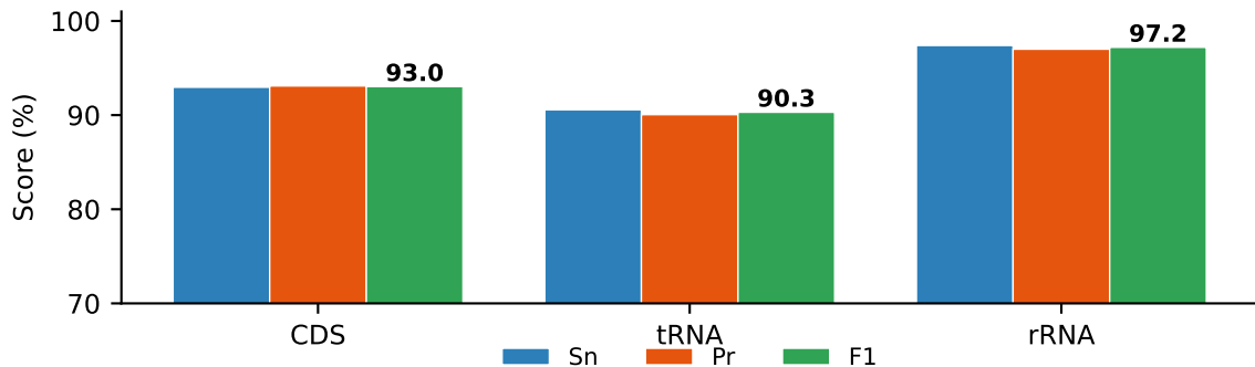
(A) Held-out accuracy by feature type
