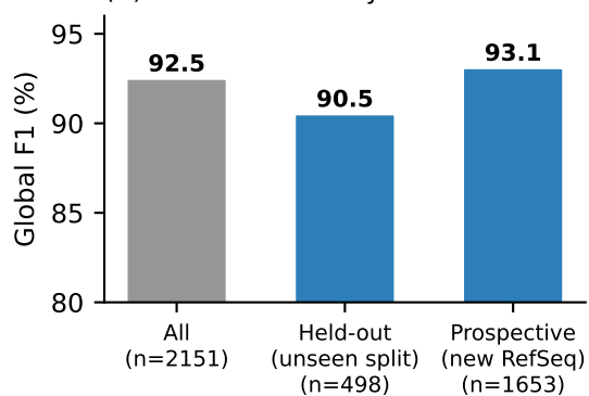
(C) Generalisation by stratum
