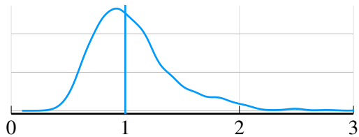
global variance \tau
