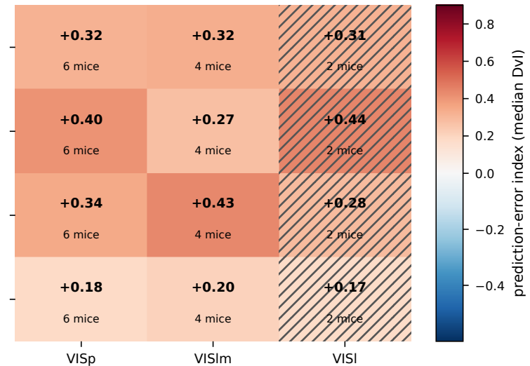
Duration / timing
