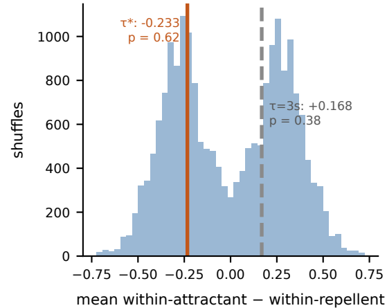
e Sign flips again; still null
