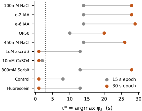
c \tau^* moves with the epoch: 0 of 10 stimuli agree
