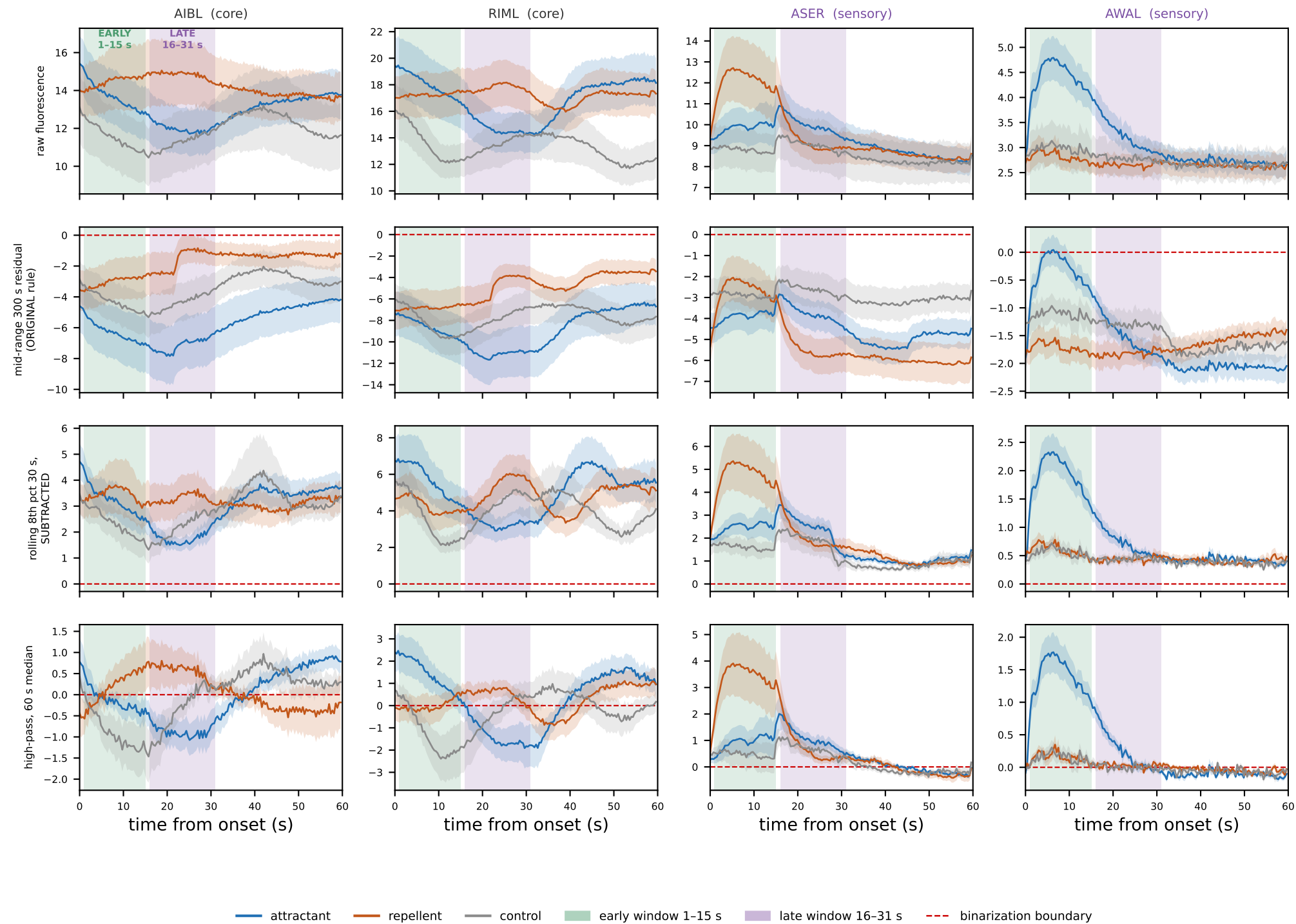
Two response windows on the 60 s stimulus cycle, mean \pm SEM (232 epochs/neuron) Sensory neurons respond in the EARLY window; core interneurons carry their class difference in the LATE window.
