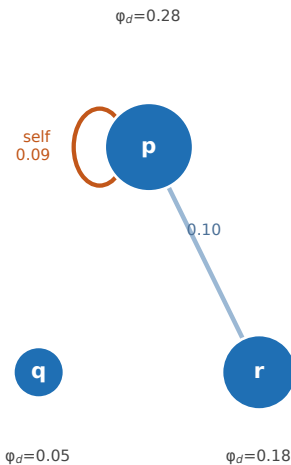
b Str2: \Phi = 0.70 3 distinctions, 2 relations (deg 1, 2)
