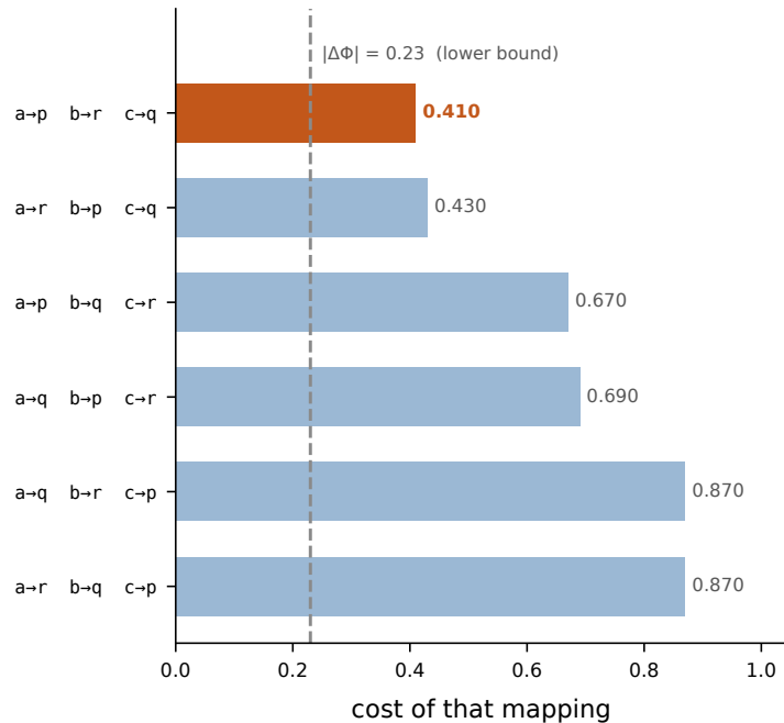
c All 3! = 6 mappings scored. D = \min = 0.410
