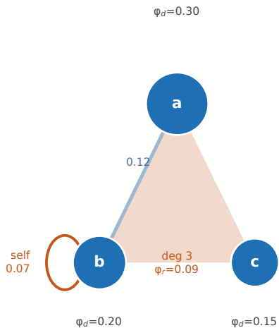
a Str1: \Phi = 0.93 3 distinctions, 3 relations (deg 1, 2, 3)
