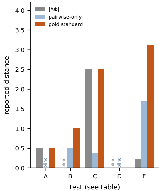
c Test D is a true isomorphism; A and B are not
