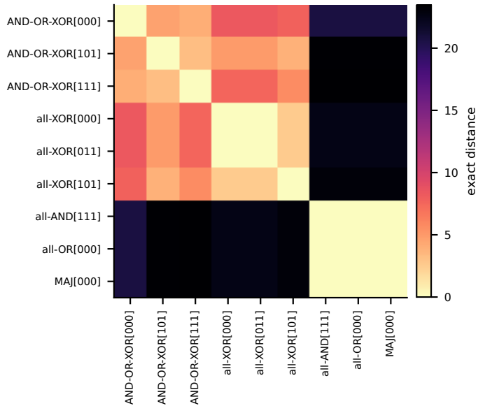
a Nine real \Phi -structures, every pair
