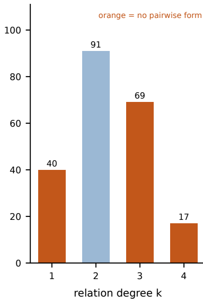
b 86 of 217 relations are degree > 2; 126 have no pairwise form
