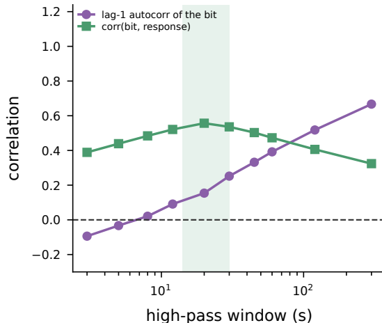
e Below ~8 s the bit anti-correlates: noise
