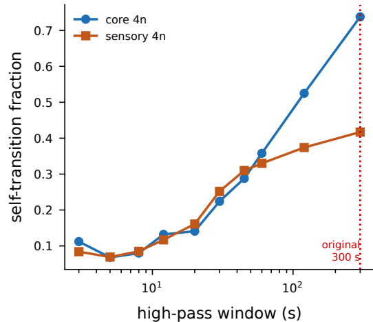
a A slow window freezes the joint state
