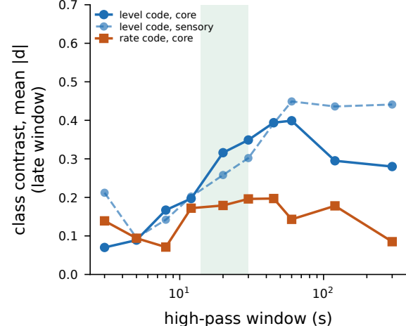
f But class coding wants a slower window
