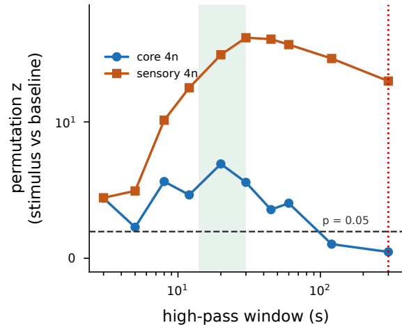
c Stimulus detectability peaks near 20 s
