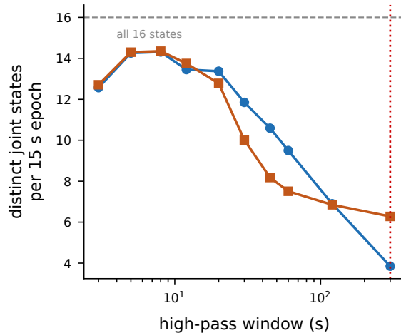
b ...and starves the TPM of state coverage
