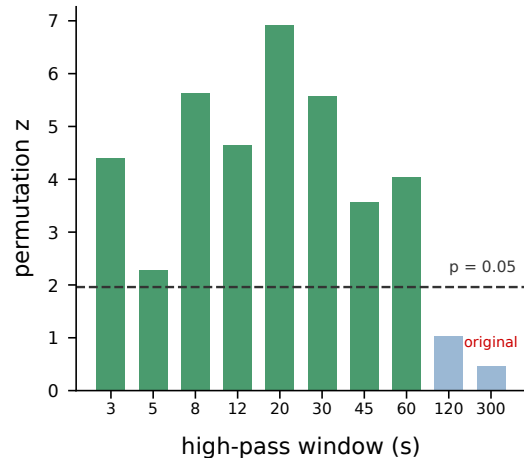
d Core quartet: z = +0.47 at 300 s, +6.92 at 20 s
