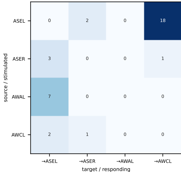
a Anatomy: synapse count (Cook 2019 via OpenWorm)
