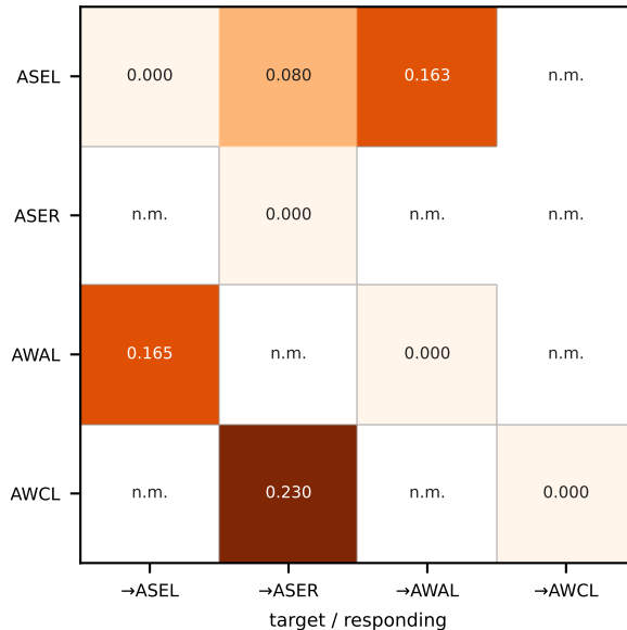
b Functional atlas: response amplitude (Randi 2023; n.m. = not measured)
