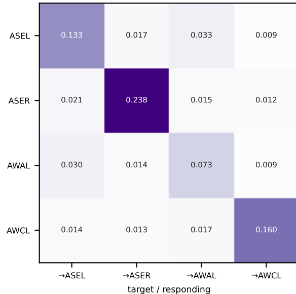
c Ours: TPM effective sensitivity (this repo, 20 s bits)
