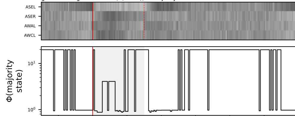
grand average of STATES (P(bit=1)) \rightarrow majority state \rightarrow \Phi
