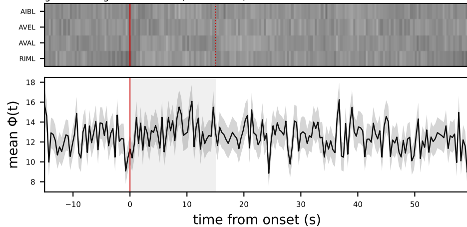
grand average of \Phi TRACES (same raster)
