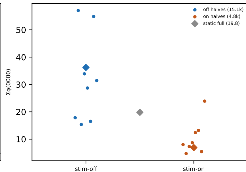
c \Sigma\phi(0000) : half-sample scatter swallows the regime gaps (dots = halves, \blacklozenge = full)
