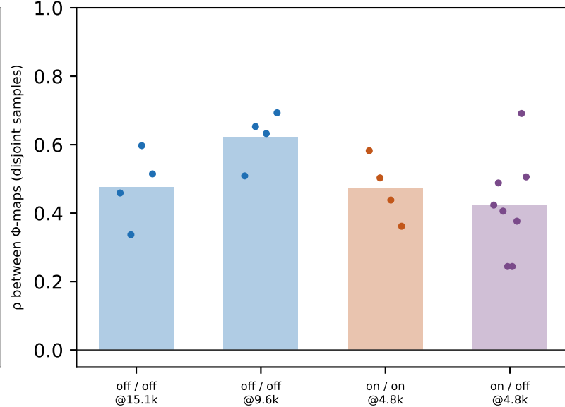
b Same-regime reproducibility \approx cross-regime agreement
