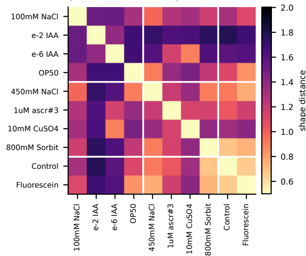
f Sensory (noise floor = 1.34)
