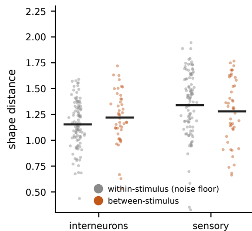
d Between-stimulus distances sit AT the within-stimulus noise floor
