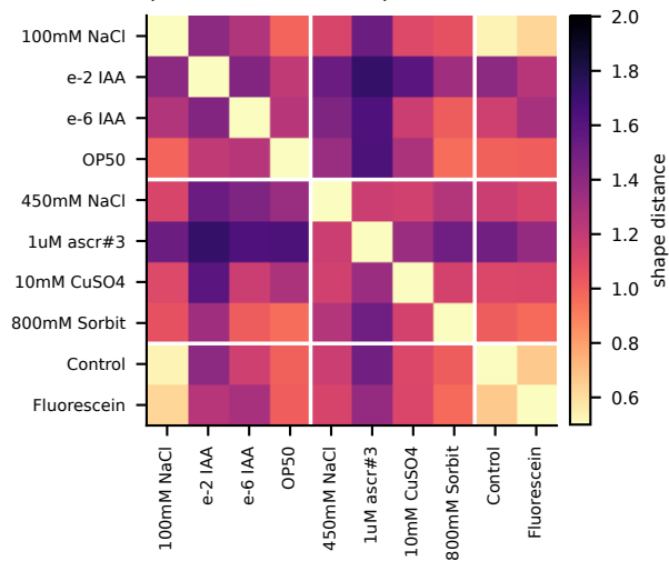
e Interneurons (noise floor = 1.15)
