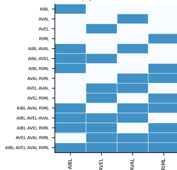
c The 15 distinction labels are the 15 non-empty subsets of the same 4 neurons
