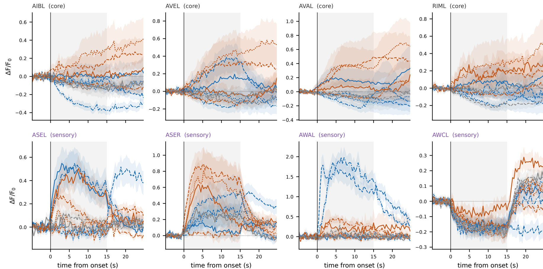
Per-stimulus responses, mean \pm SEM of \Delta F/F_0 — all 8 animals — variance across the 24 epochs of each stimulus
