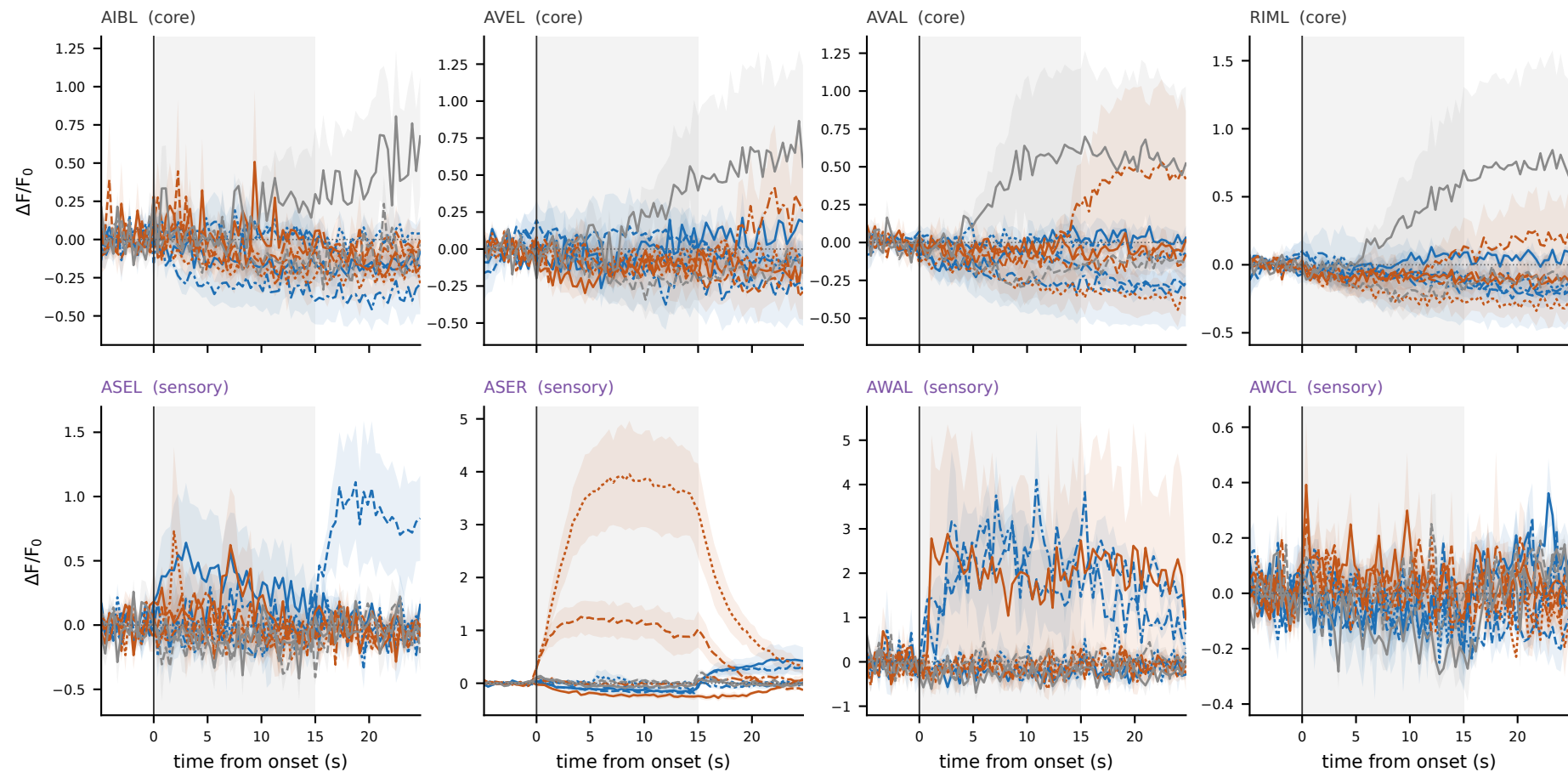
Per-stimulus responses, mean \pm SEM of \Delta F/F_0 — one animal (20220327_herm_2) — variance across the 3 repeats of each stimulus
