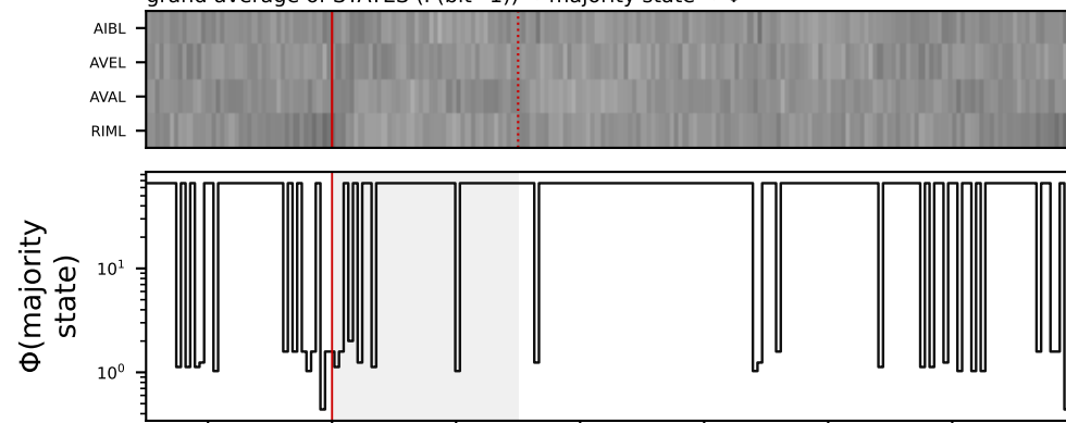
grand average of STATES (P(bit=1)) \rightarrow majority state \rightarrow \Phi
